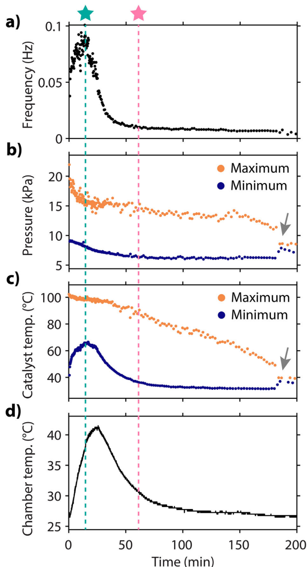
FIGURE 3 | Evolution in time of the active oscillations. Evolution over more than 3 consecutive hours of (a) the oscillation frequency, (b) the maximum and minimum values of the oscillating pressure, (c) the maximum and minimum values of the oscillating catalyst temperature, and (d) the temperature inside the chamber. Grey arrows in (b) and (c) denote the transition to a small-amplitude oscillation.
