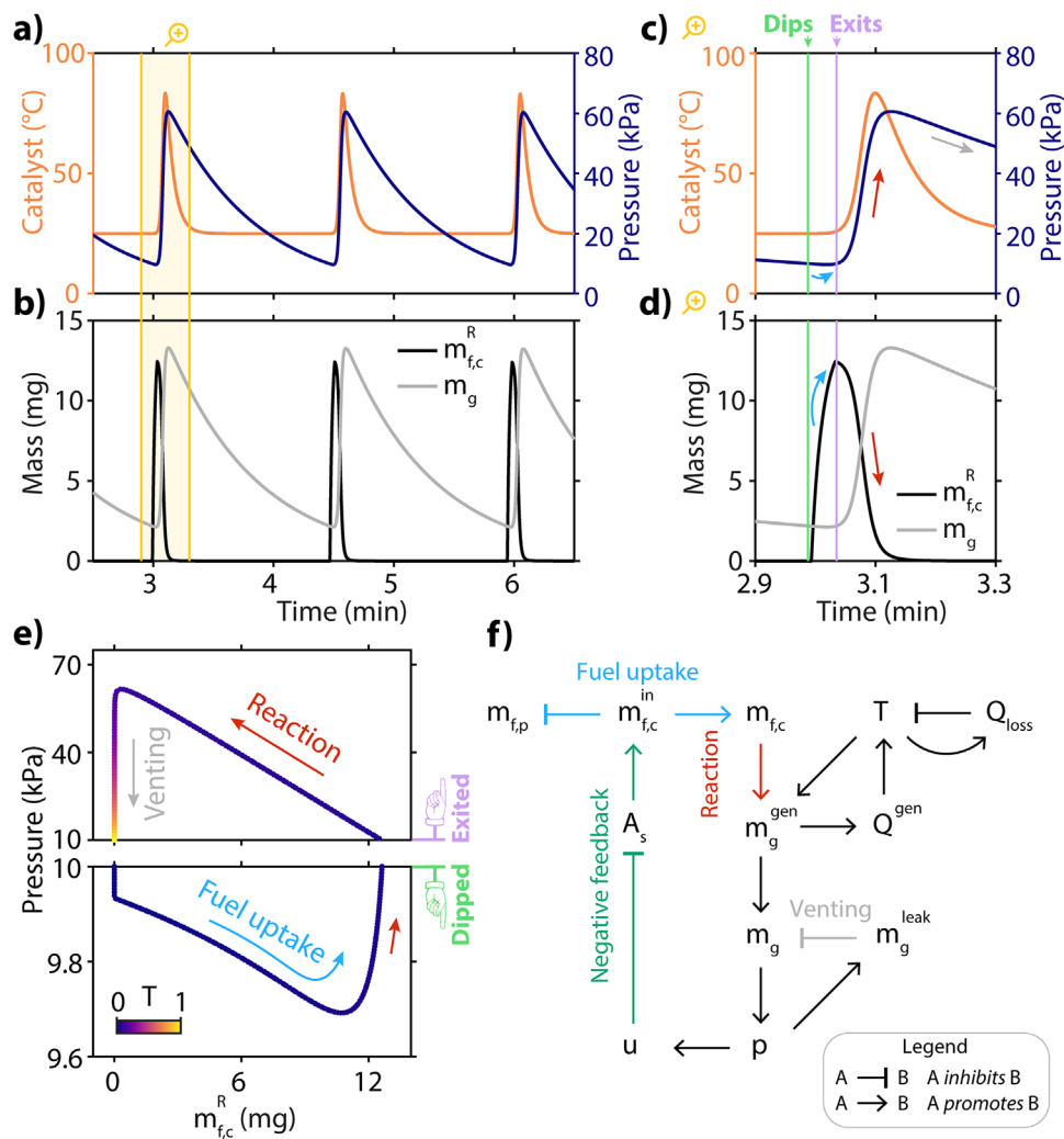
FIGURE 5 | The model captures the active oscillation. (a) Evolution in time of the catalyst temperature (orange) and the chamber pressure (blue) of the modeled system (third to fifth inflation cycles). (b) Evolution in time of the mass of reactable fuel in the catalyst (black) and the mass of gas in the chamber (gray) of the modeled system (third to fifth inflation cycles). (c, d) A zoomed view of the third inflation cycle highlights when the catalyst enters the pool (green) and when the catalyst exits the pool (purple), defined as the instants when the catalyst displacement moves past the fuel pool surface (Supplementary Materials). (e) Hysteresis highlighted by a period of oscillation ( T : 0 to 1) displayed in the domain of reactable fuel in the catalyst m_{f,c}^R versus pressure. (f) We represent how the key variables in the model qualitatively affect each other. Flat arrowheads from a variable A to a variable B indicate that A inhibits B. Pointy arrowheads from variable A to variable B indicate that A promotes B. We highlight in blue the effective fuel uptake into the catalyst, causing an increase in the mass of fuel in the catalyst m_{f,c}^R . In red, we indicate the catalytic reaction that generates a mass of gas m_g^{\text{gen}} from the mass of fuel in the catalyst m_{f,c}^R . In grey, we indicate how the gas that vents to atmosphere reduces the mass of gas in the chamber. In green, we indicate the effect of negative feedback, for which an increase in displacement u causes a decrease in the surface area of contact A_s of the catalyst with the fuel in the pool, inhibiting fuel uptake into the catalyst. The parameters used in these simulations are listed in Table S1.
