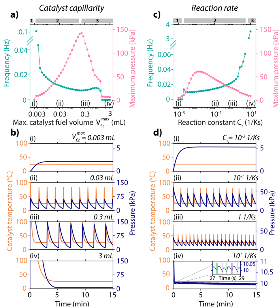
FIGURE 7 | Influence of catalyst capillarity and reaction constant on the active oscillation. (a) Frequency (green) and maximum pressure (pink) of the active oscillation when varying the maximum volume of fuel in the catalyst V_{f,c}^{max} from 3 \mu\text{L} to 3 \text{ mL} . The three regimes are highlighted with grey bars, with numbers 1, 2, and 3. (b) Catalyst temperature (orange) and pressure (blue) for the four key cases (i–iv) in (a). (c) Frequency (green) and maximum pressure (pink) of the active oscillation when varying the reaction constant C_r from 1 \times 10^{-3} 1/Ks to 1 \times 10^1 1/Ks. The three regimes are highlighted with grey bars, with numbers 1, 2, and 3. (d) Catalyst temperature (orange) and pressure (blue) for the four key cases (i–iv) in (c). The inset in (iv) highlights the high-frequency oscillation occurring over 2 s, with the catalyst oscillating at low amplitude around the pool level, rapidly entering (green) and exiting (purple) the pool. All simulation parameters (apart from the varied ones) are listed in Table S1.
