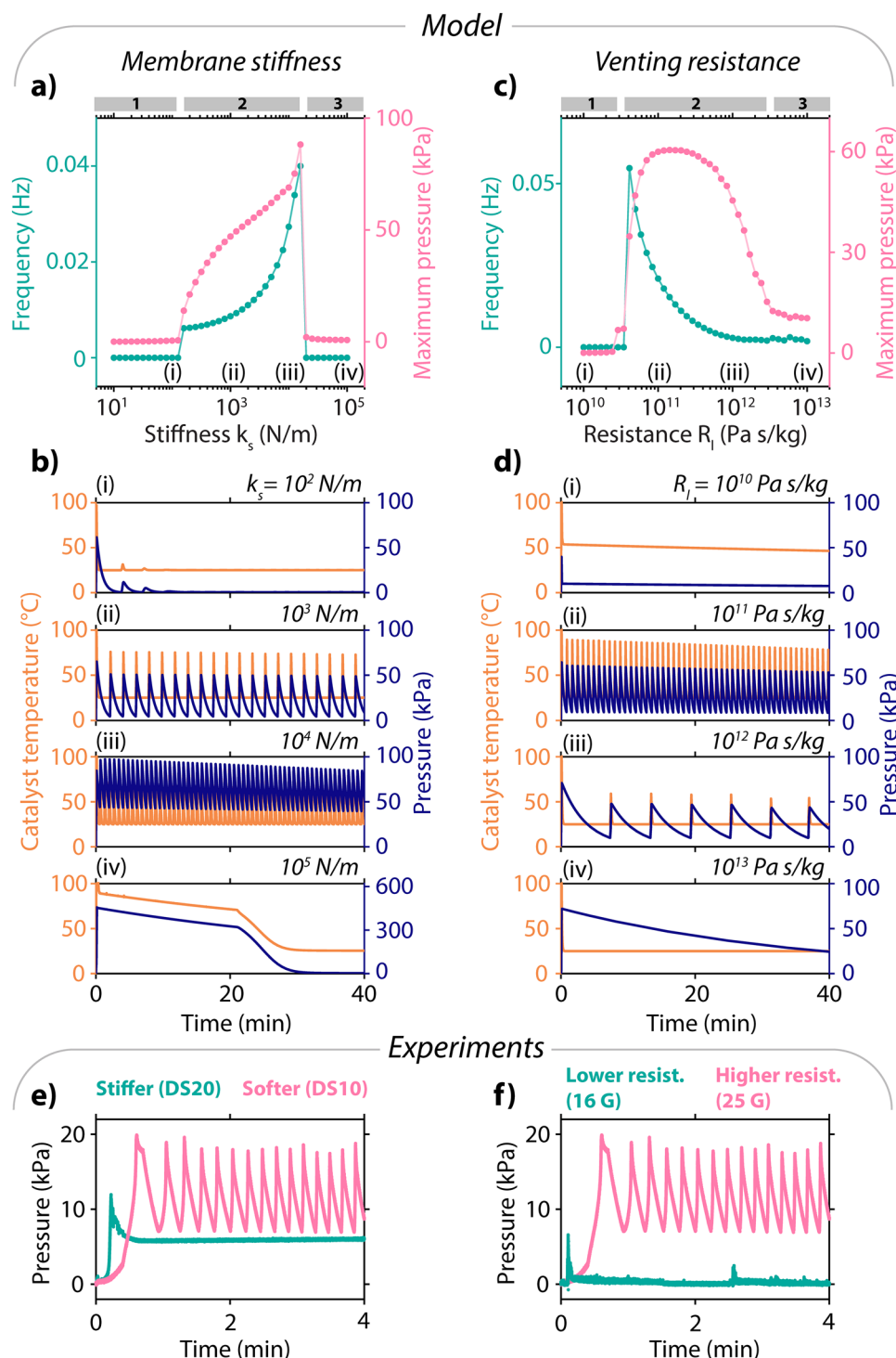
FIGURE 6 | Influence of membrane stiffness and venting resistance on the active oscillation. (a) Frequency (green) and maximum pressure (pink) of the active oscillation when varying the membrane stiffness k_s from 1 \times 10^1 N/m to 1 \times 10^5 N/m. The three regimes are highlighted with grey bars, with numbers 1, 2, and 3. (b) Catalyst temperature (orange) and pressure (blue) for the four key cases (i–iv) in (a). (c) Frequency (green) and maximum pressure (pink) of the active oscillation when varying the venting resistance R_l from 1 \times 10^{10} Pa s/kg to 1 \times 10^{13} Pa s/kg. The three regimes are highlighted with grey bars, with numbers 1, 2, and 3. (d) Catalyst temperature (orange) and pressure (blue) for the four key cases (i–iv) in c. All simulation parameters (apart from the varied ones) are listed in Table S1. When frequency is zero, we define the maximum pressure as the pressure value at the end of the test, at time 40 min. (e) Experimental evolution in time of the pressure in the active oscillator with a stiffer membrane with Young's modulus \sim 0.621 MPa (Smooth-On DS20) (green) and with a softer membrane with Young's modulus \sim 0.237 MPa (Smooth-On DS10) (pink), given the same venting resistance (25 G needle). (f) Experimental evolution in time of the pressure in the active oscillator with a lower venting resistance (16 G needle) (green) and with a higher venting resistance (25 G needle) (pink), given the same membrane (Smooth-On DS10). Pink datapoints in e and f are the same experiment (DS10 membrane and 25 G needle).
