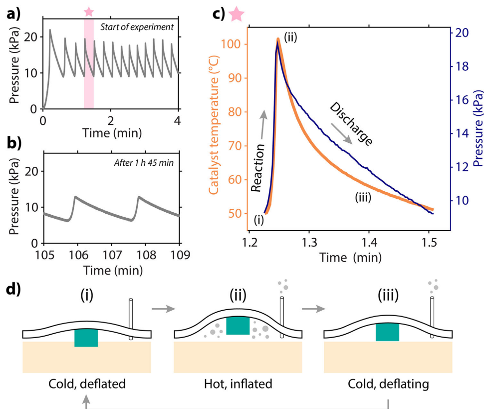
FIGURE 2 | The active oscillator spontaneously inflates and deflates for hours. (a) Active oscillations occurring in the first 4 min of the experiment. (b) After 1 h and 45 min, the active oscillation is still self-sustaining, with a lower frequency and at lower pressures. (c) The trends of the temperature at the catalyst and of the pressure during the fourth oscillation cycle (pink star in a) highlight a reaction phase followed by a discharge phase. (d) Schematics of three stages of the oscillation cycle: (i) the catalyst is cold and dipped in the fuel, as the membrane is deflated, (ii) the catalyst is hot and the membrane is inflated as the reaction occurred, and (iii) the gases are venting to atmosphere, the membrane is deflating, and the catalyst is cooling down.
