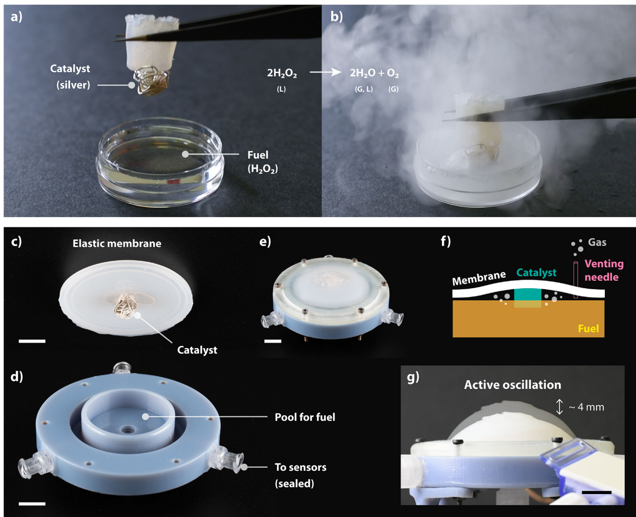
FIGURE 1 | An active fluidic oscillator with embodied energy. (a) When a catalyst (50 cm of silver wire with diameter 0.5 mm) enters in contact with fuel (liquid hydrogen peroxide, 50 % concentration in water), (b) the fuel rapidly decomposes releasing gas (water vapor and oxygen) and residual liquid water. The fuel stores energy (with energy density \sim 1.44 kJ/g, one order of magnitude higher than lithium-ion batteries [30]) which is released in gas, and hence can be directly used to power pneumatic systems. (c) We partially embed the silver wire catalyst in an elastic membrane, leaving the majority of the surface area of the wire exposed (Supplementary Materials). (d) The fuel (6 mL in volume) is contained in a 3D-printed rigid holder, with three ports for insertion of two temperature sensors and a pressure sensor (Supplementary Materials). (e) The membrane is clamped on top of the fuel pool, with the catalyst facing the pool. (f) A needle is connected to one of the ports to vent the gases generated during the reaction. (g) The membrane exhibits active oscillations, alternatively inflating and deflating as a consequence of the reaction activating and deactivating cyclically. Scale bars in c, d, e, and g are 1 cm.
