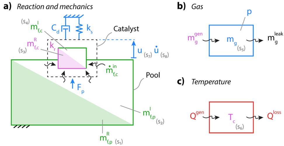
FIGURE 4 | Schematic of the model of the active oscillator. (a) We model the pool as a volume of fuel with a reactable part m_{f,p}^R (green) and an inert part m_{f,p}^I (white). The catalyst is also modeled as a container of fuel, with a reactable part m_{f,c}^R (purple) and an inert part m_{f,c}^I (white). Fuel exchanges between the pool and the catalyst (black arrows), with rate \dot{m}_{f,c}^{\text{in}} . Only the reactable fuel in the catalyst is assumed to decompose into gases, with a reaction rate k_r function of the temperature of the catalyst T_c . The catalyst is attached to a linear spring with stiffness k_s and a damper with damping coefficient C_d , and it moves upwards by a displacement u under the force F_p generated by the pressurized gas. (b) The mass of gas generated through the reaction \dot{m}_g^{\text{gen}} increases the total mass of gas inside the chamber m_g , inducing pressurization p . The gas leaking through the venting needle \dot{m}_g^{\text{leak}} reduces the mass of gas in the chamber. (c) The temperature of the catalyst T_c increases due to the heat Q^{\text{gen}} generated by the exothermic reaction and decreases due to heat losses Q^{\text{loss}} . We denote the state variables as s_i , with i = 1 to 8 .
